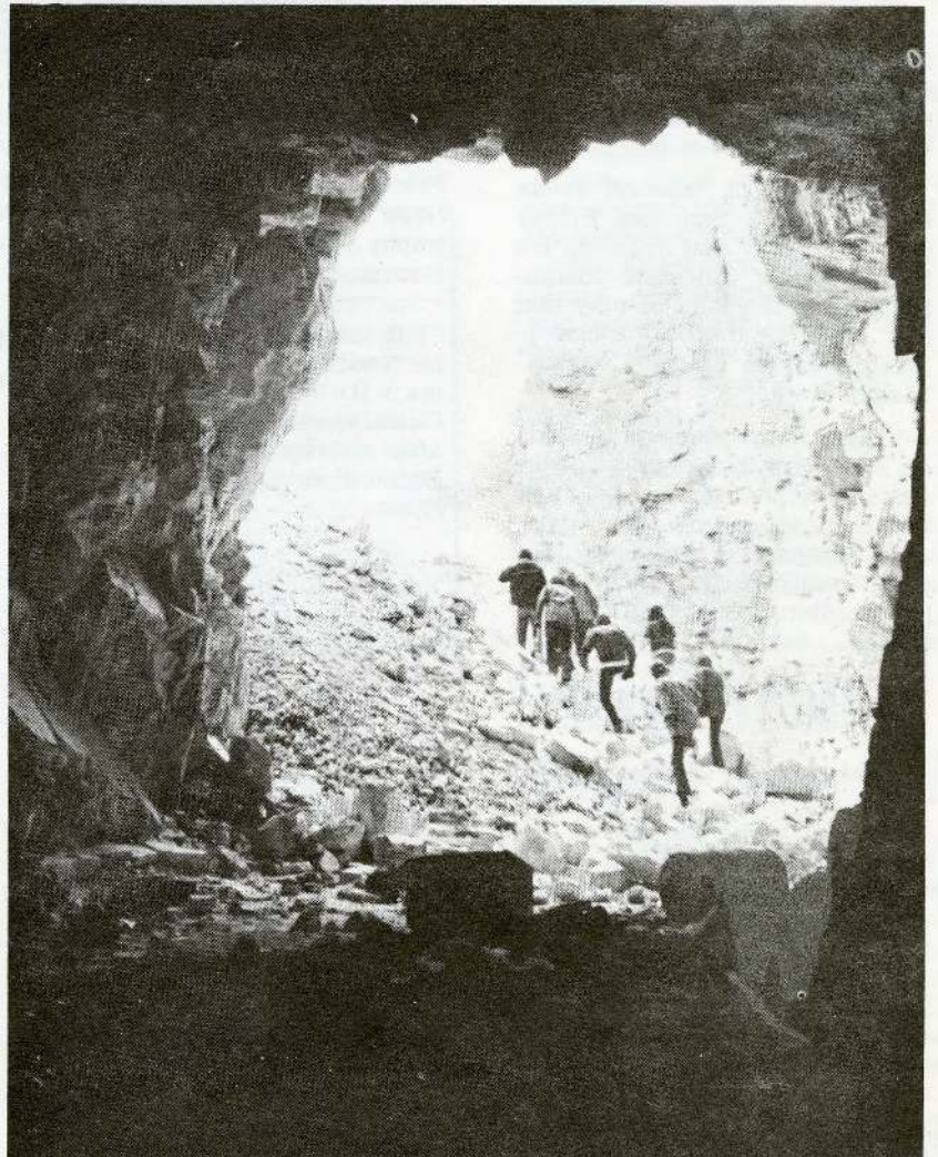
The geology field trip included inspection of mammoth dolomite marble mine near Lone Pine. Student guests raised over-all total on trip to more than 100.
