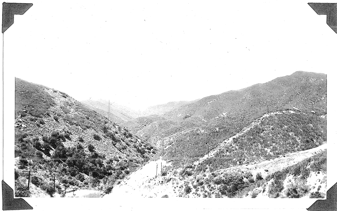
West in Clearwater Canyon. Clearwater fault between granite on the right and Martinez(?) sandstones on the left. Los Angeles Municipal Power house #1 in the foreground.
